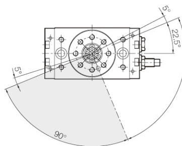
● 90° 迴轉 Swing rotation
