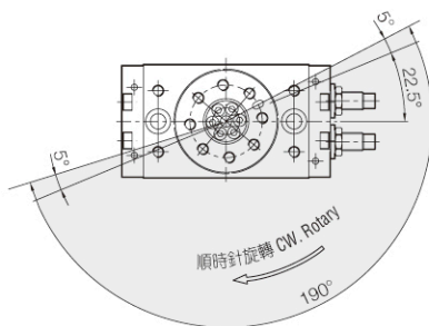
● 190° 迴轉 Swing rotation
