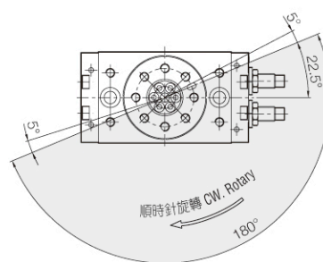
● 180° 迴轉 Swing rotation
