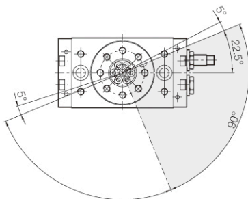
● 90° 迴轉 Swing rotation
