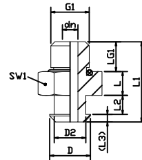
連接部件SC 030/040... EH,適用於VFM-1.5 20...30 Connecting parts SC 030/040 ... EH, suitable for VFM-1.5 20 ... 30
