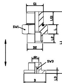
連接部件SC 050 G1/4-M,適用於VFM-1.5 40...50 Connecting parts SC 050 G1 / 4-M for VFM-1.5 40 ... 50
