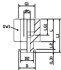
連接部件SC 040 G1/8-F,適用於VFM-1.5 20...30 Connecting parts SC 040 G1 / 8-F for VFM-1.5 20 ... 30
