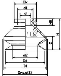
連接部件SC 040 G1/8-F,適用於VFM-1.5 20...30 Connecting parts SC 040 G1 / 8-F for VFM-1.5 20 ... 30
